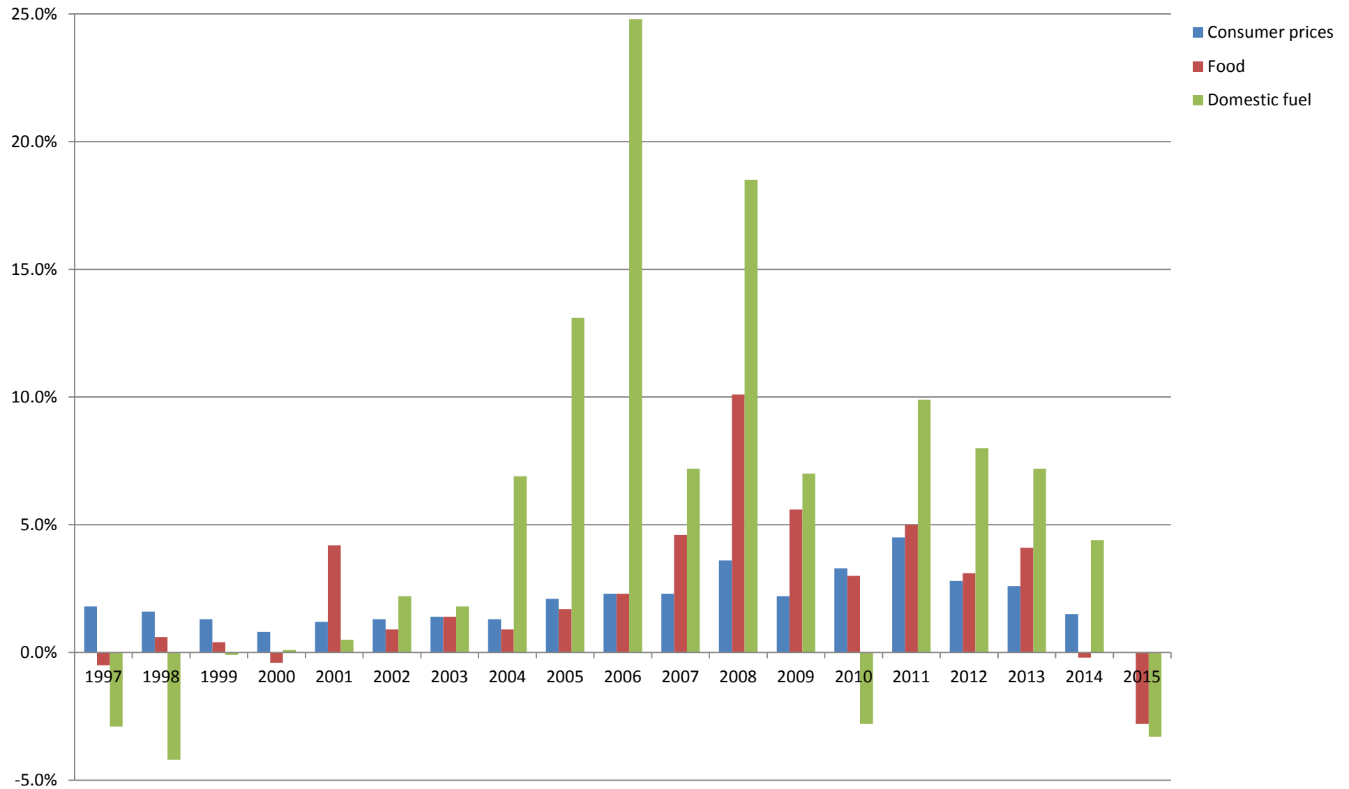
Figure 2 Inflation rates: annual changes in Consumer Prices Index and the cost of food and home energy, 1997-2015
